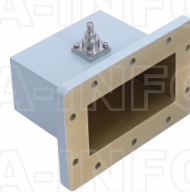
430WCAS Right Angle Rectangular Waveguide to Coaxial Adapter 1.7-2.6GHz WR430 to SMA Female
